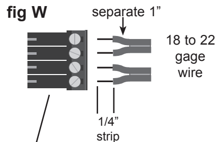
Control voltage wire preparation for screw terminals
