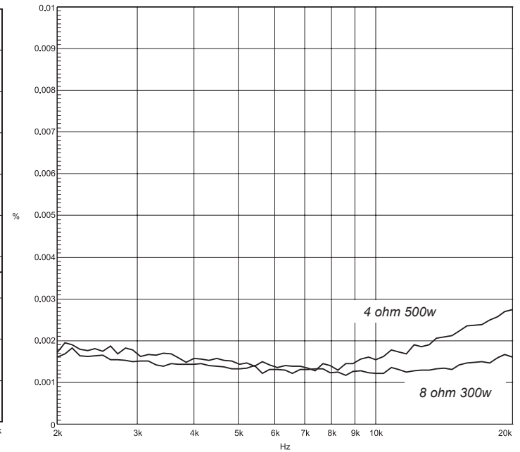
Typical IMD Sweep 4BSST
