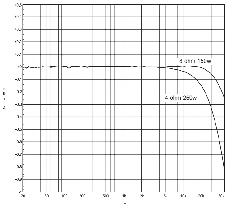
Typical Frequency Response 3BSST
