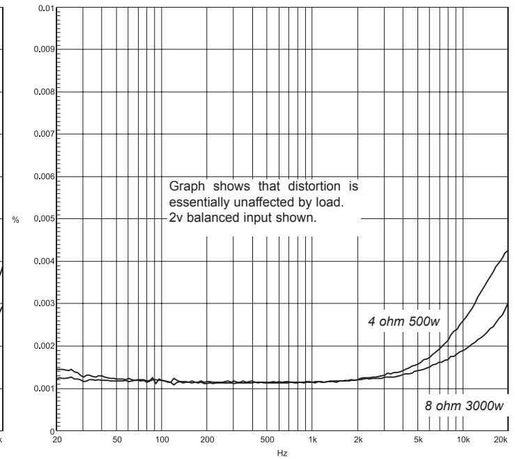
Typical THD+N Sweep 4BSST
